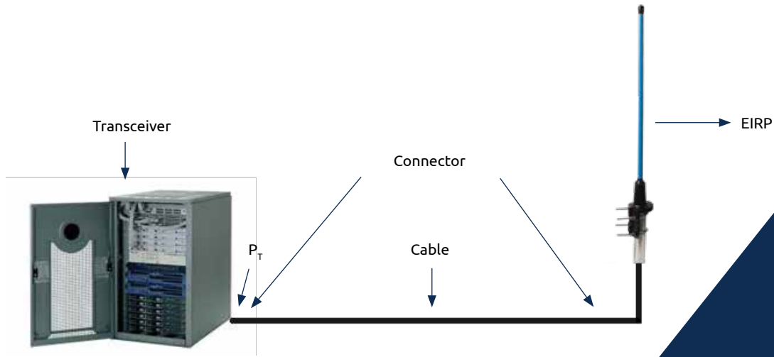
Determining the EIRP of an RF transmitting system
